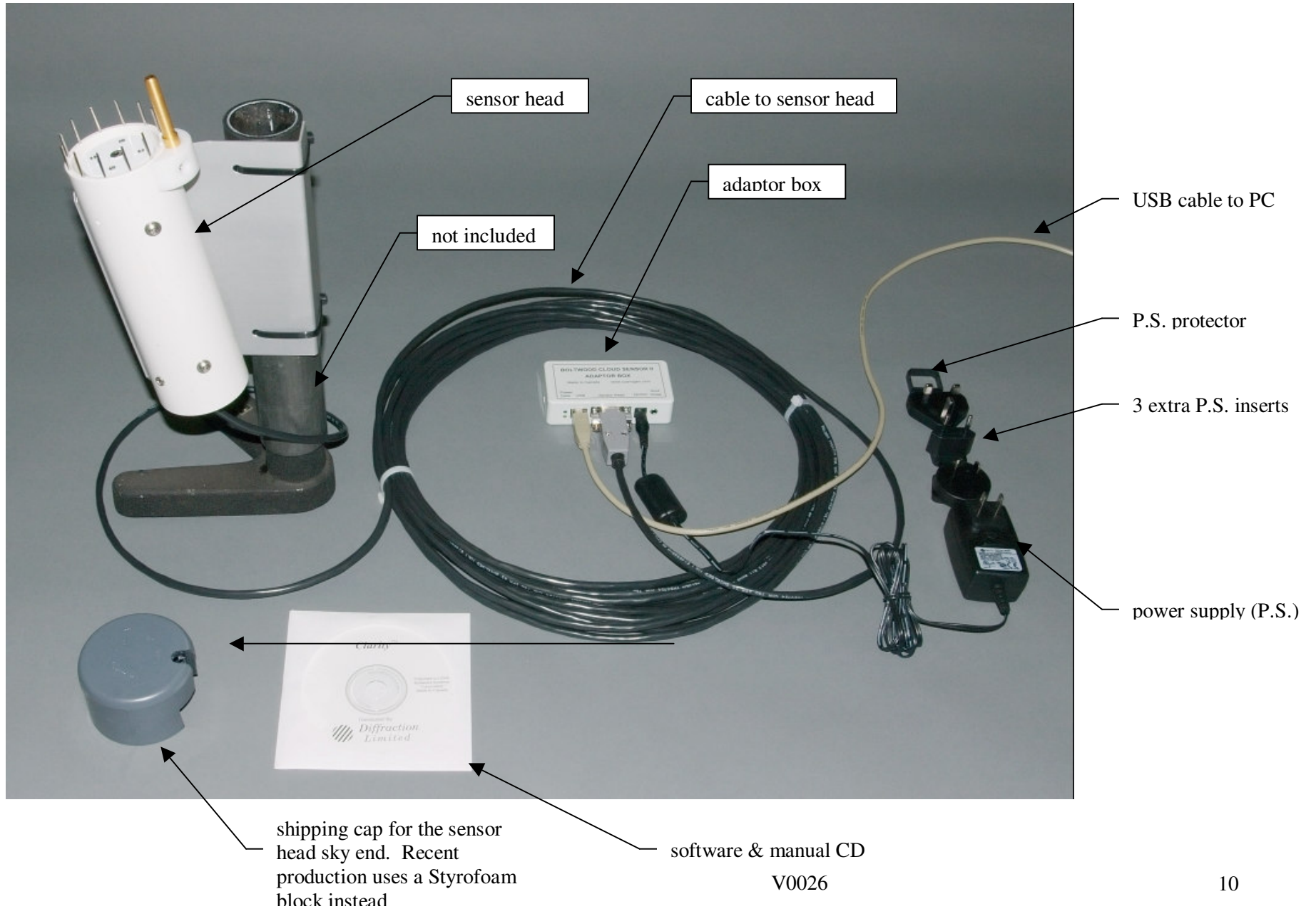
Figure 3 - Cloud Sensor II System Parts
