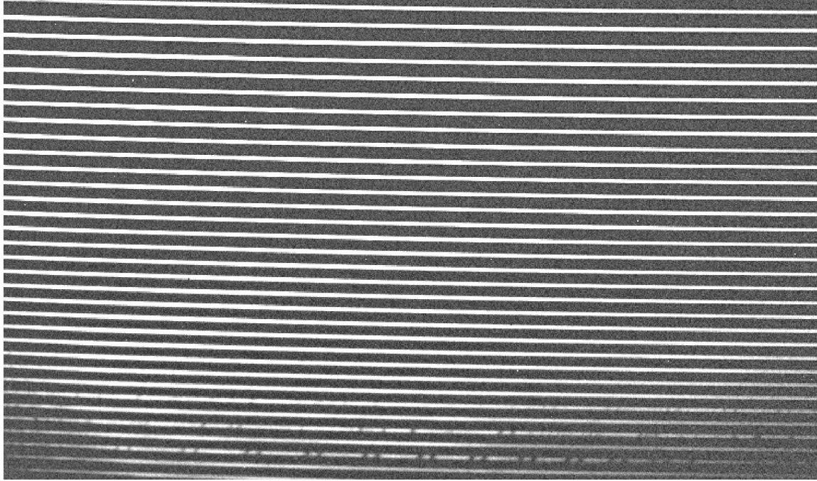
Part of the spectrum of Vega, 5 minute exposure. Red orders are on the bottom. Telluric absorption bands are visible in the red.
