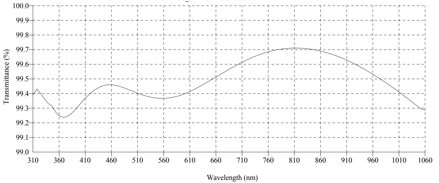
JS_1LAF3: Transmittance
