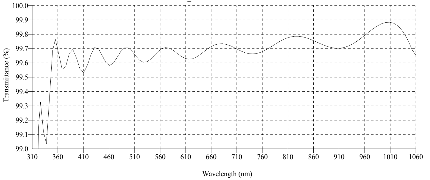
FUS_SIL3: Transmittance
