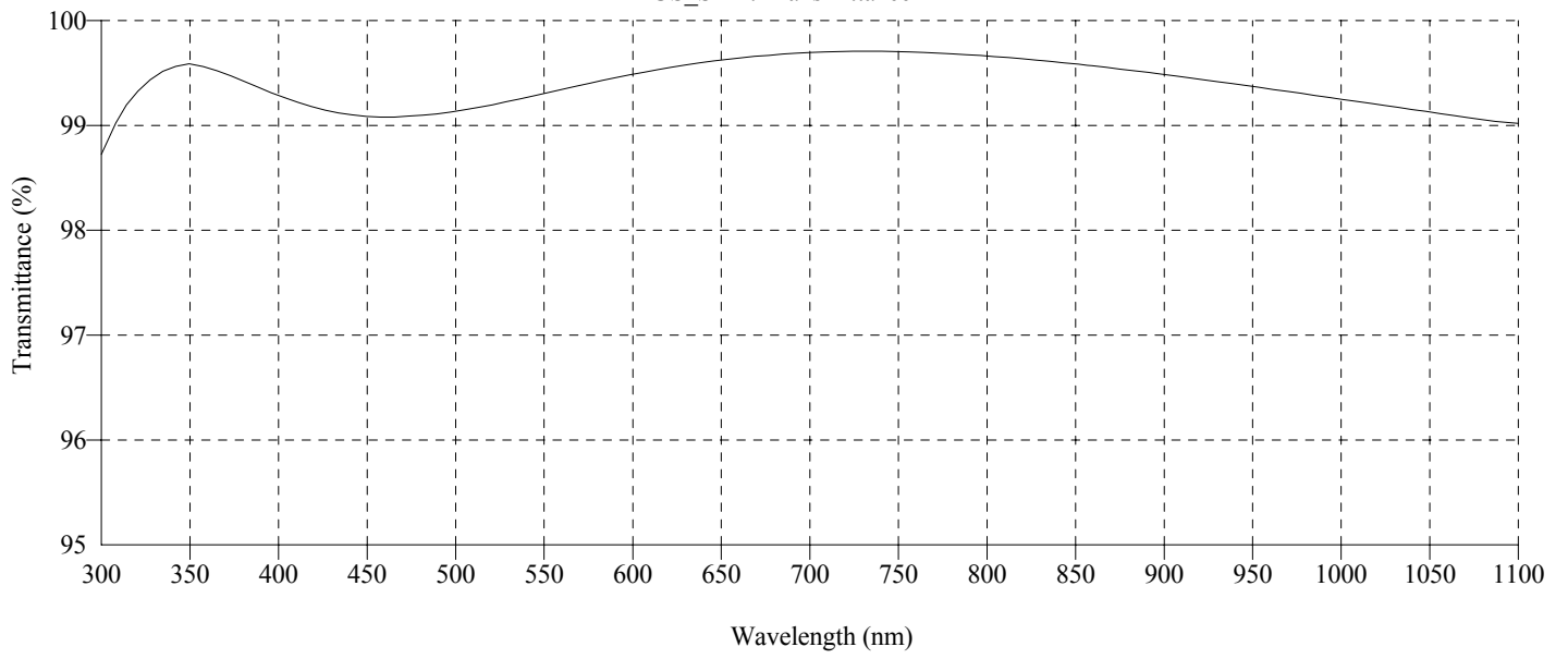
FUS_SIL2: Transmittance
