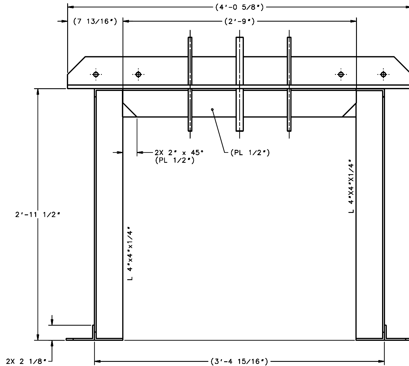
SECTION F-F (SHT 3) SCALE 1:4
