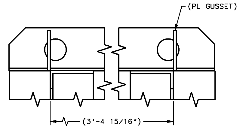
SECTION E-E (SHT 2) SCALE 3:8 ROTATED 90° CW
