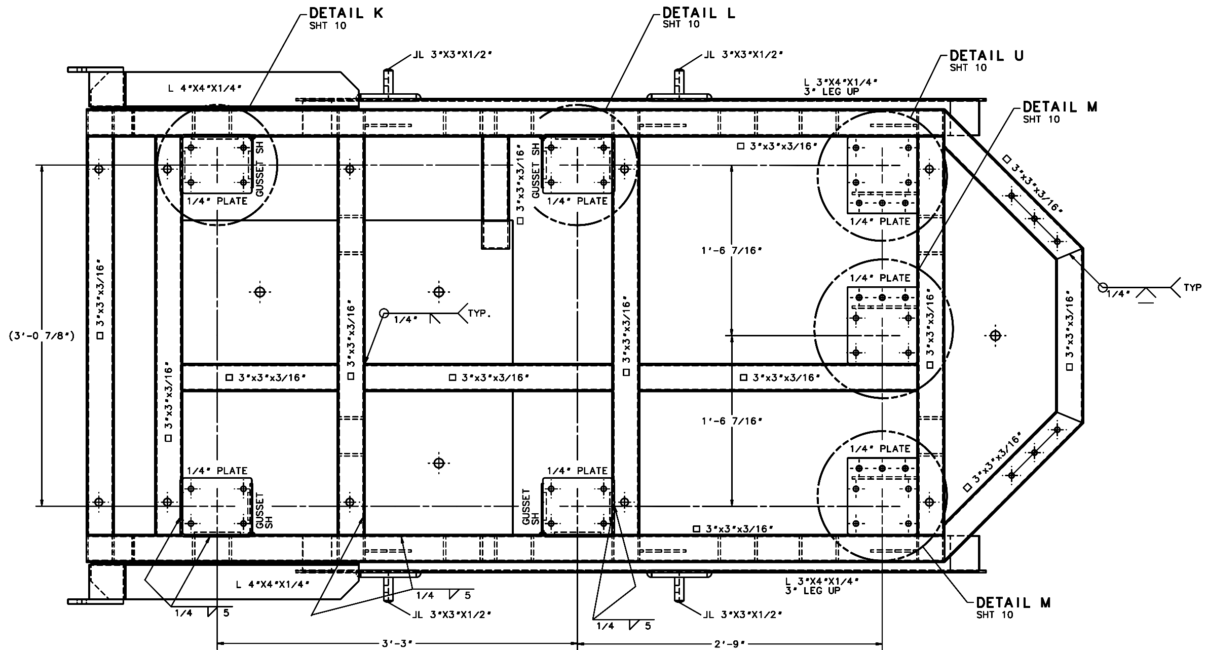
VIEW P-P SHT 2 SCALE 3:16 WHEELS NOT SHOWN
