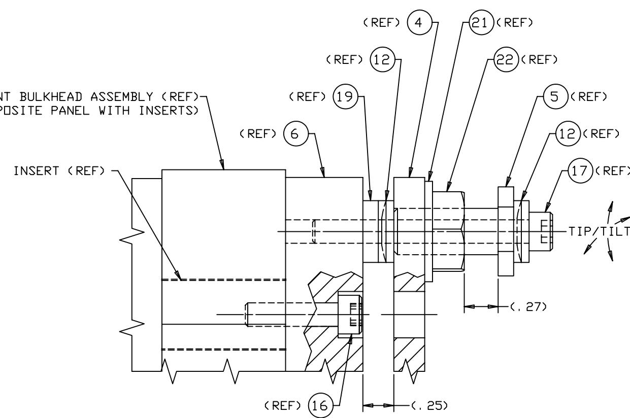
DETAIL B (THIS SHT) SCALE 2.5: 1
