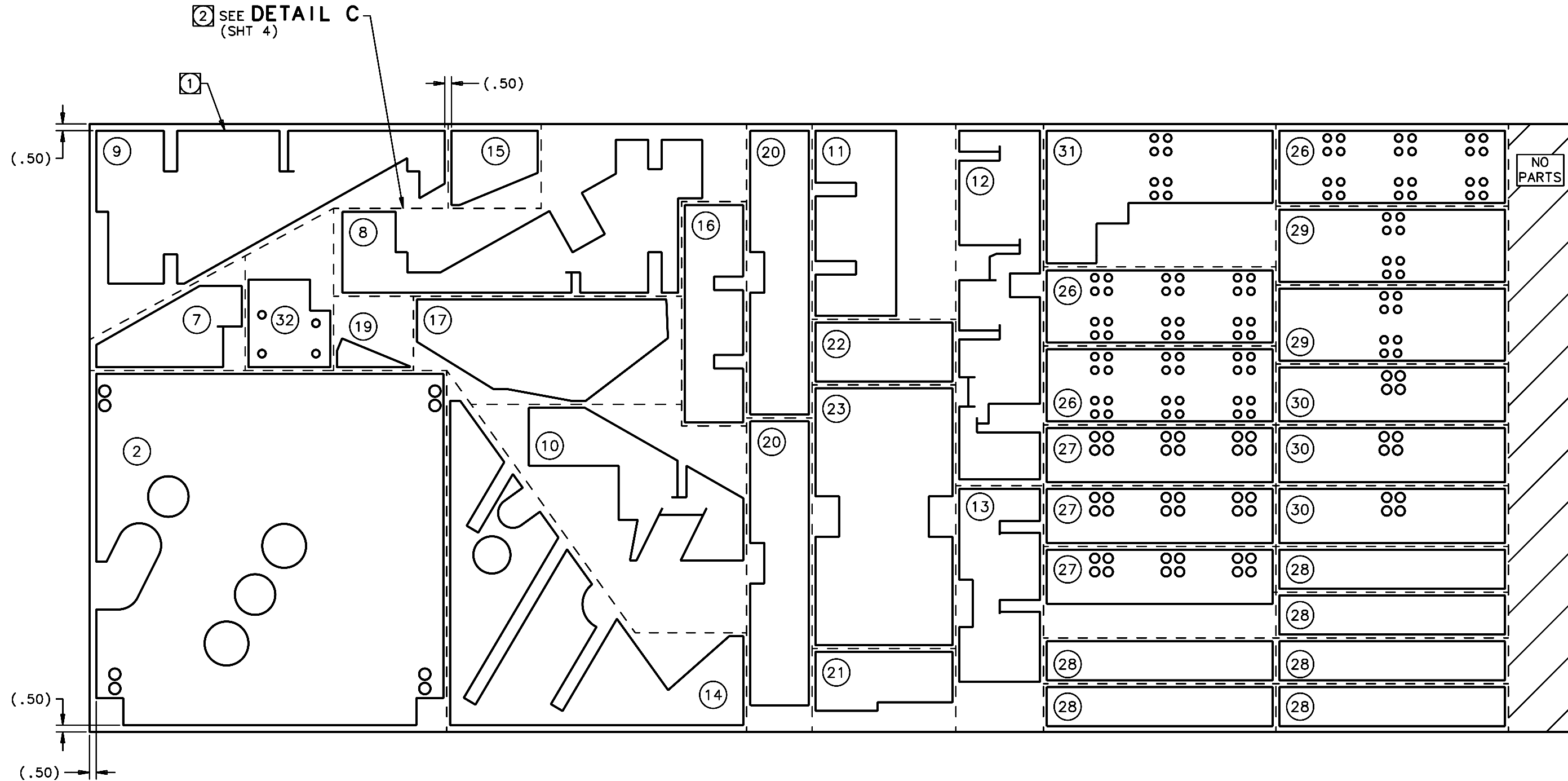
DETAIL A (SHT 1) SCALE 1:4 PARTS LAYOUT
