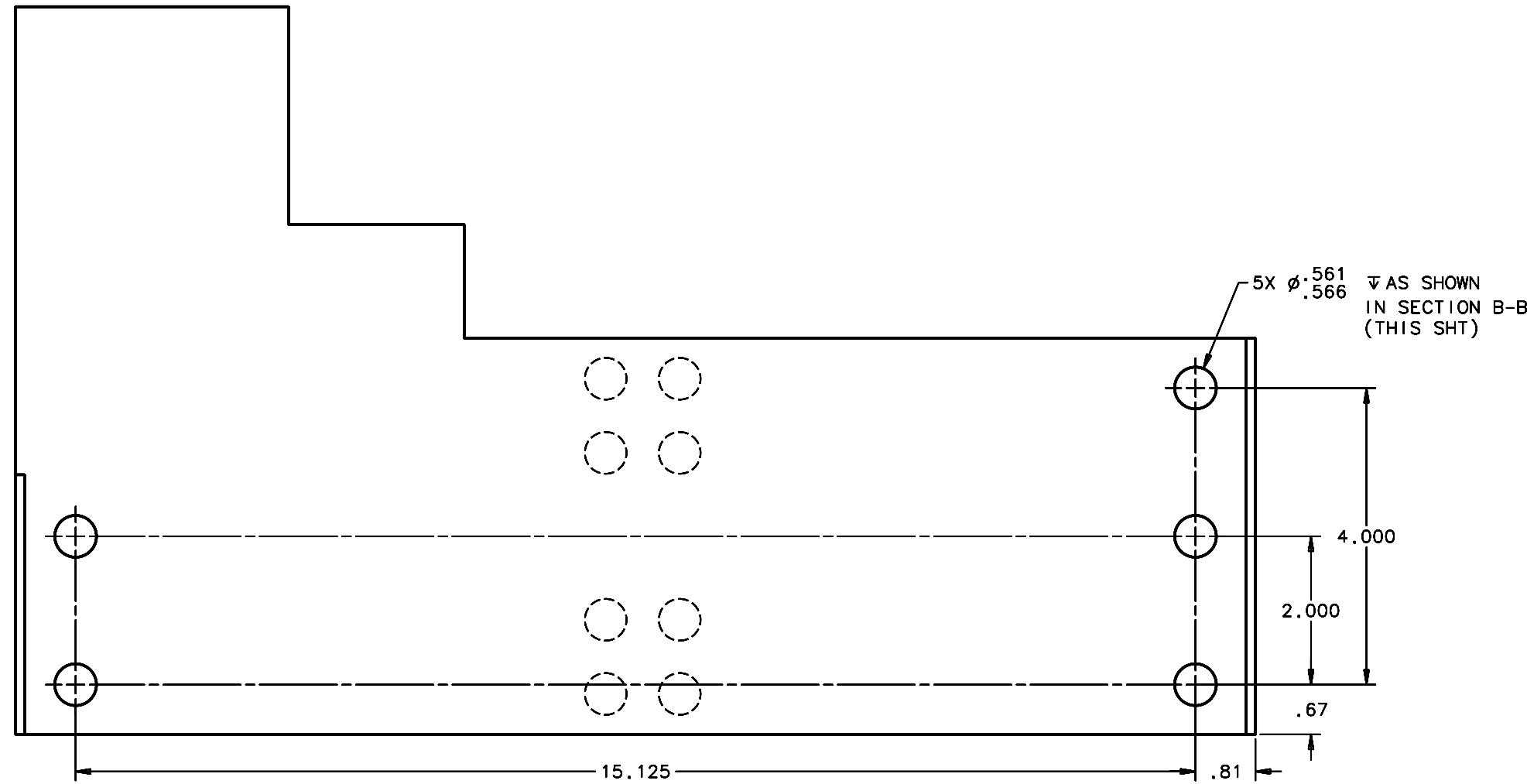
VIEW A-A (SHT 1) SCALE 1:1
