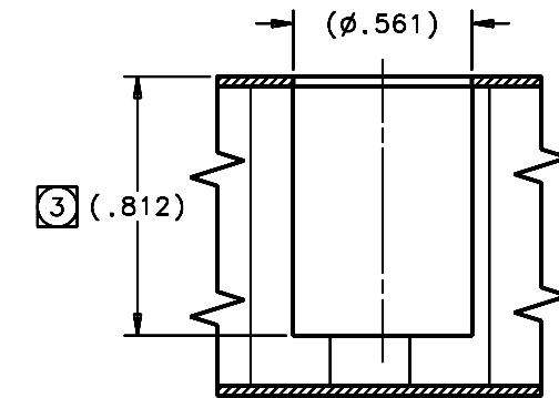
SECTION B-B (SHT 1) SCALE 3:1
