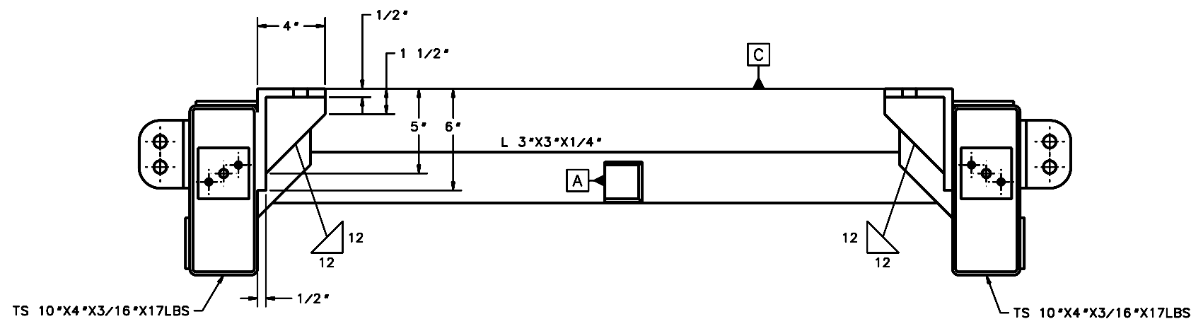
SECTION J-J SHT 4 SCALE 1:4 ALL DIMENSIONS TYP WHERE APPLICABLE
