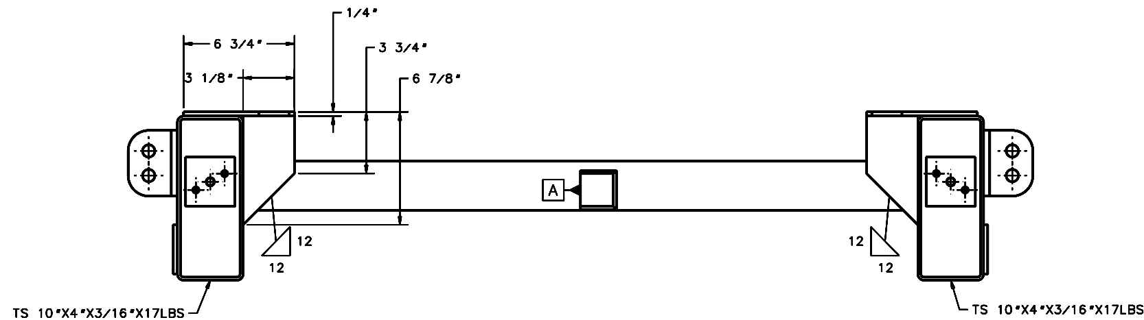
SECTION H-H SHT 4 SCALE 1:4 ALL DIMENSIONS TYP WHERE APPLICABLE
