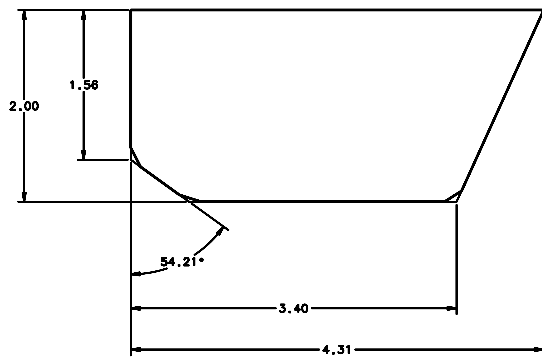
⑥ INJECTION OPTICS MOUNTING BOX PLATE 6
