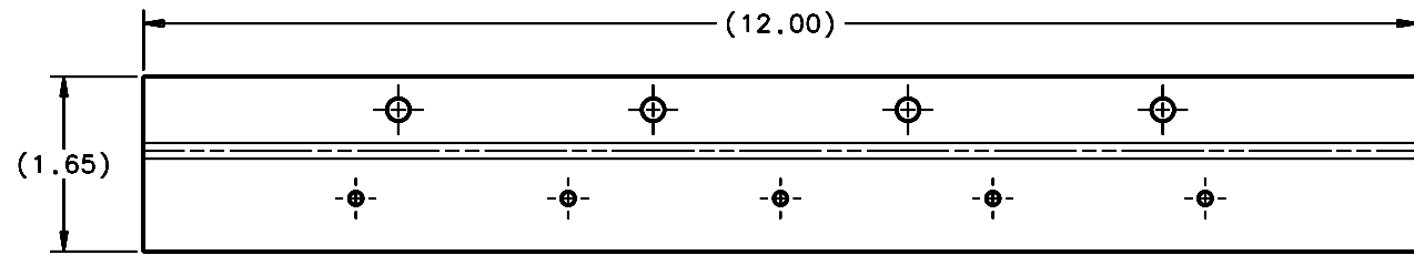
FLAT PATTERN SCALE 1:1 FOR REF ONLY
