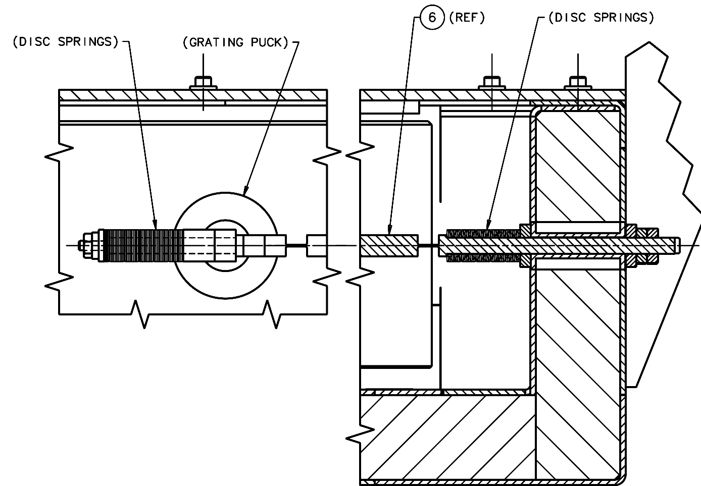
SECTION B-B (SHT 4) SCALE 1 3/4:1
