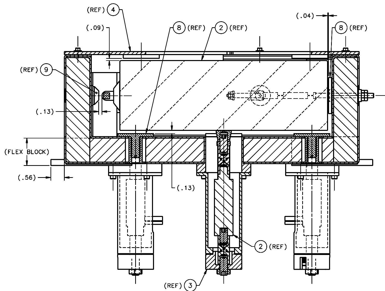
SECTION A-A (SHT 4) SCALE 1:1
