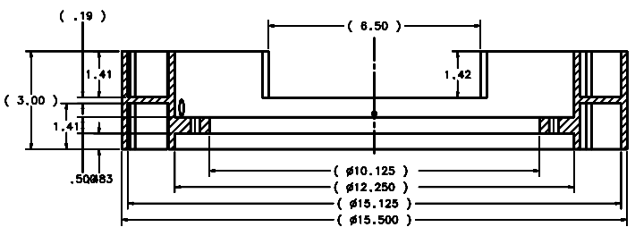
SECTION F-F SHT 2 SCALE .75:1
