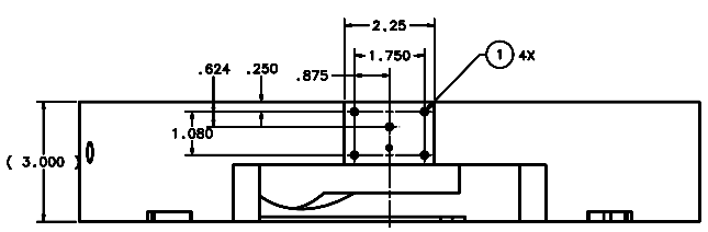
VIEW G-G SHT 3 SCALE .75:1
