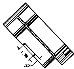
SECTION R-R SHT 3 SCALE .75:1
