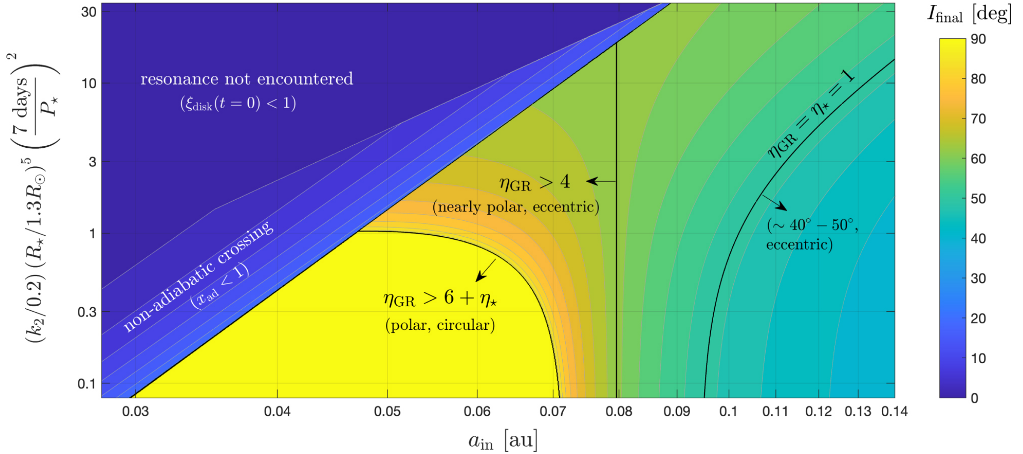
Figure 4. from A Disk-driven Resonance as the Origin of High Inclinations of Close-in Planets null 2020 APJL 902 L5 doi:10.3847/2041-8213/abb952 http://dx.doi.org/10.3847/2041-8213/abb952 © 2020. The American Astronomical Society. All rights reserved.
