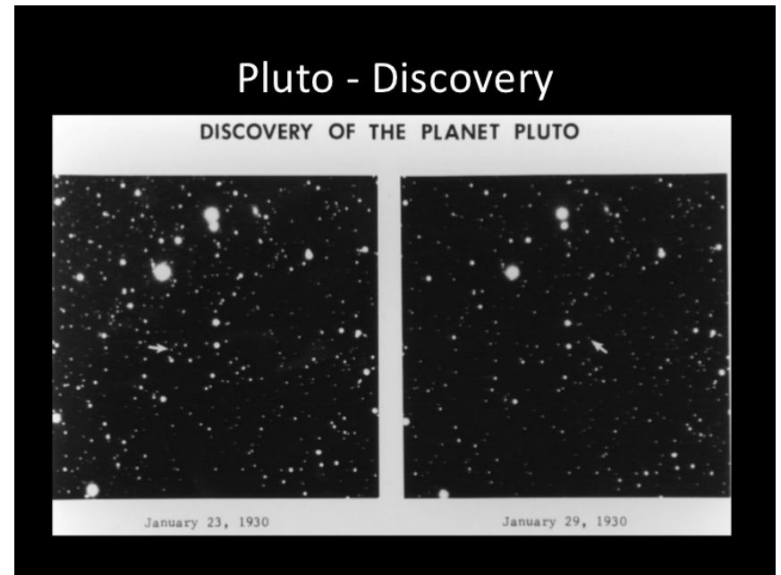
Discovery of Pluto
