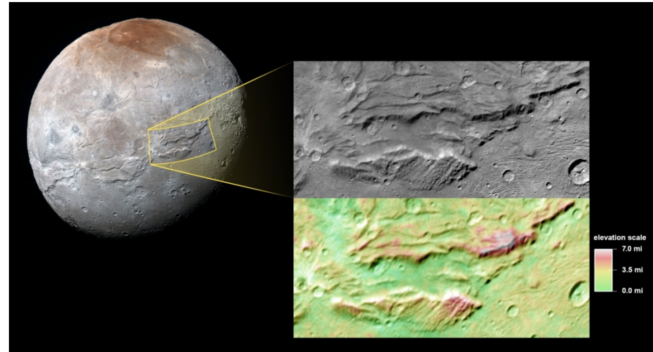
Charon
