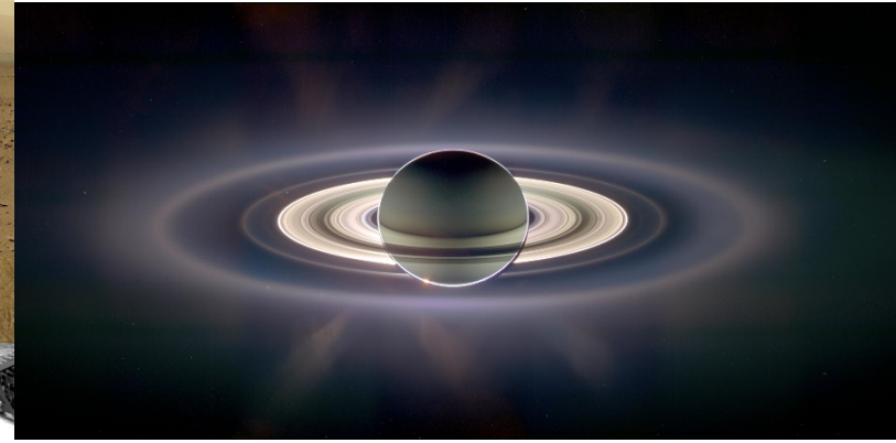
Saturn
