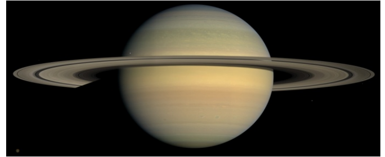
Saturn
