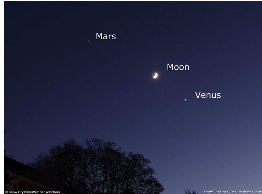
Mars and Venus with the Moon
