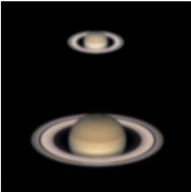
Saturn
